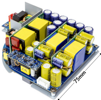
Ultra Low Noise GaN Power with Active Noise Cancellation
